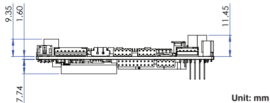
Figure 5: PCM-3365 Mechanical Drawing (Side View, W/O heatsink)
