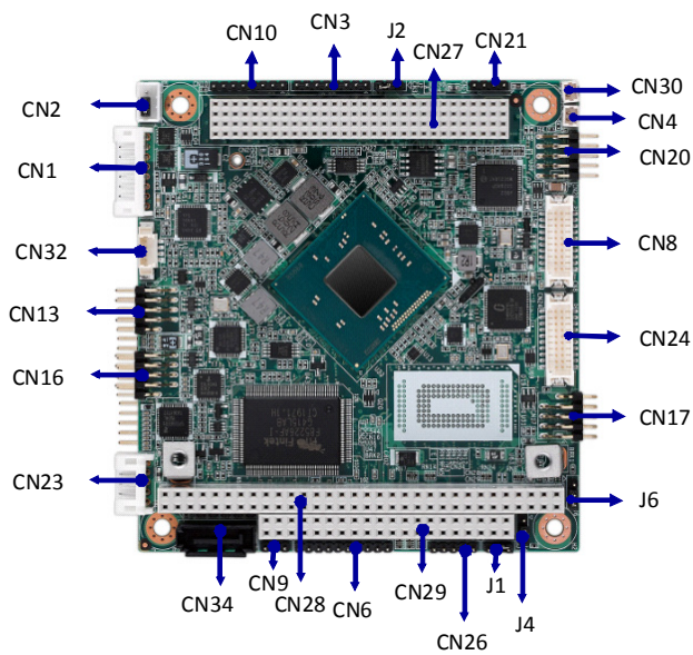
Figure 1: PCM-3365 Connector Location (Top Side)
