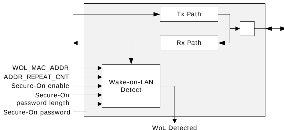
Figure 17 • Wake-on-LAN Functionality
