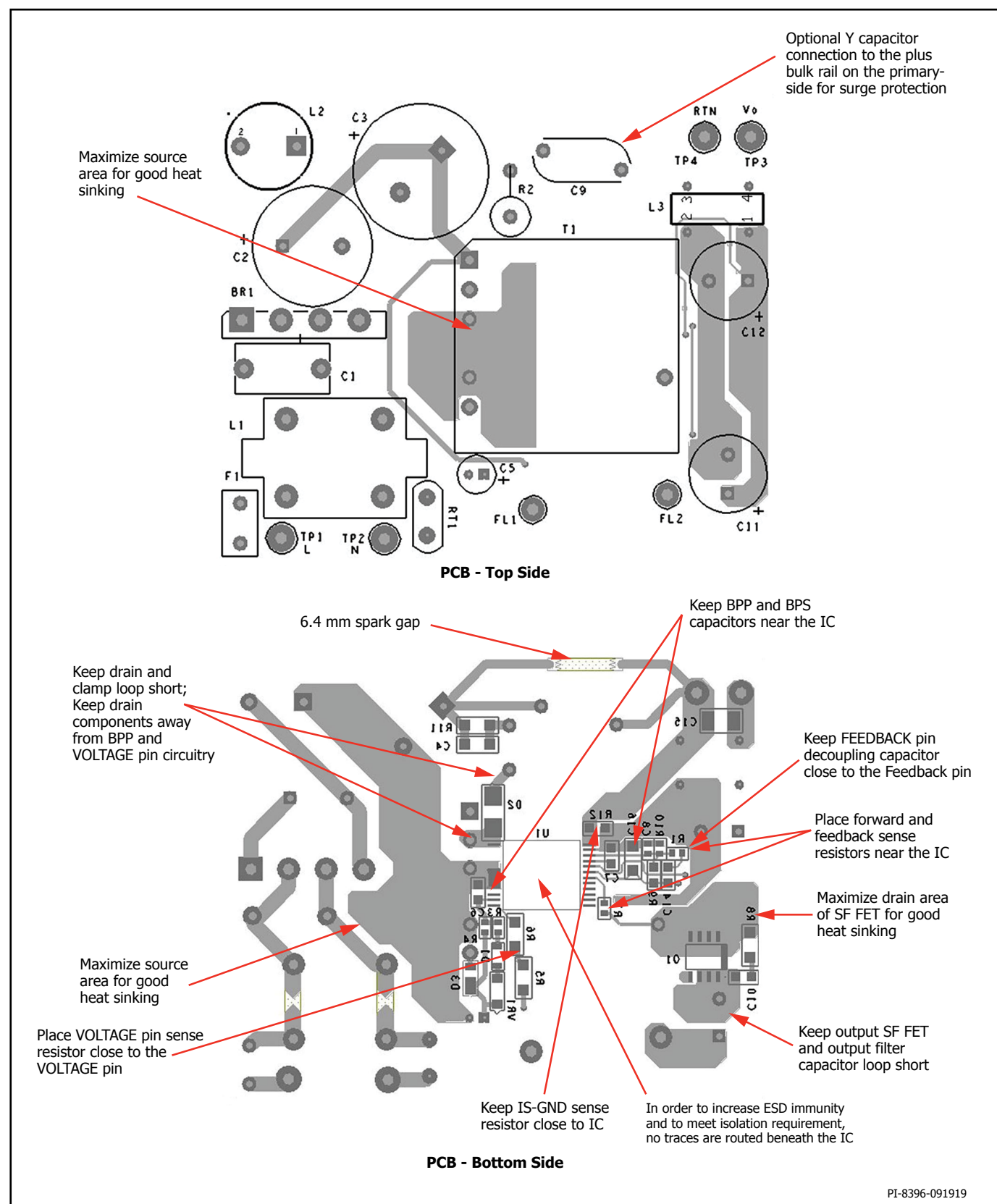
Figure 18. PCB.
