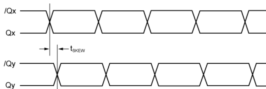
Figure 3. Output-to-Output Skew
