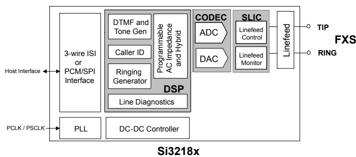
Si3218x Functional Block Diagram
