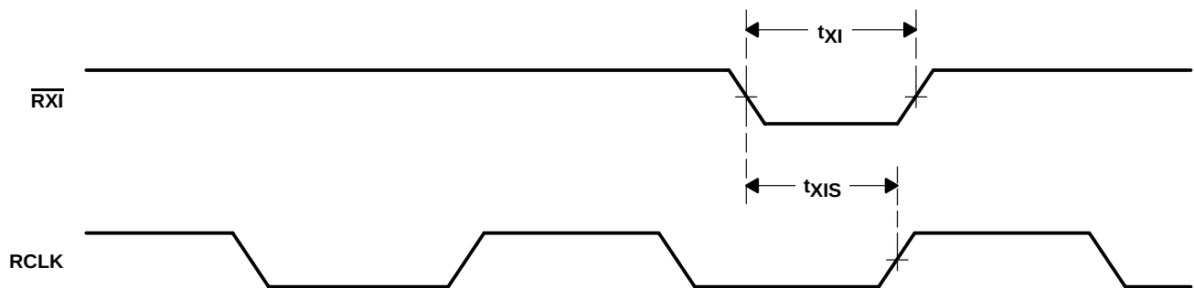
Figure 15. Read-Expansion-In Timing
