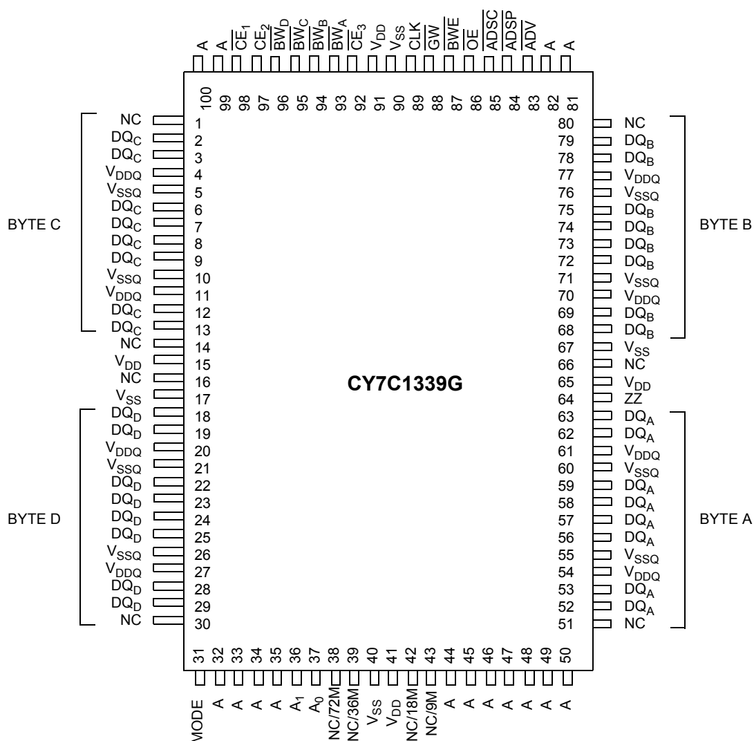
Figure 1. 100-pin TQFP (14 × 20 × 1.4 mm) pinout [1]
