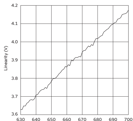
Graph 2 When the connection impedance is 200\text{k}\Omega
