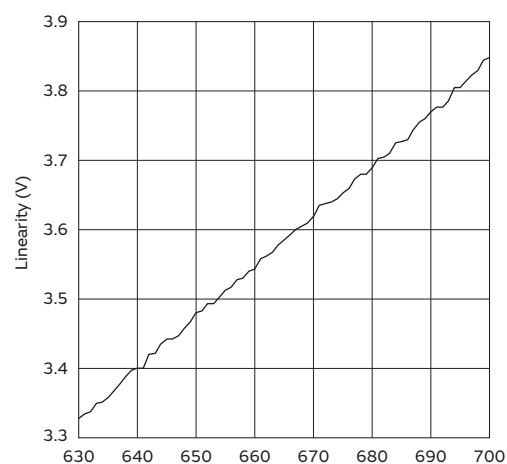
Graph 1 When the connection impedance is 1\text{M}\Omega
