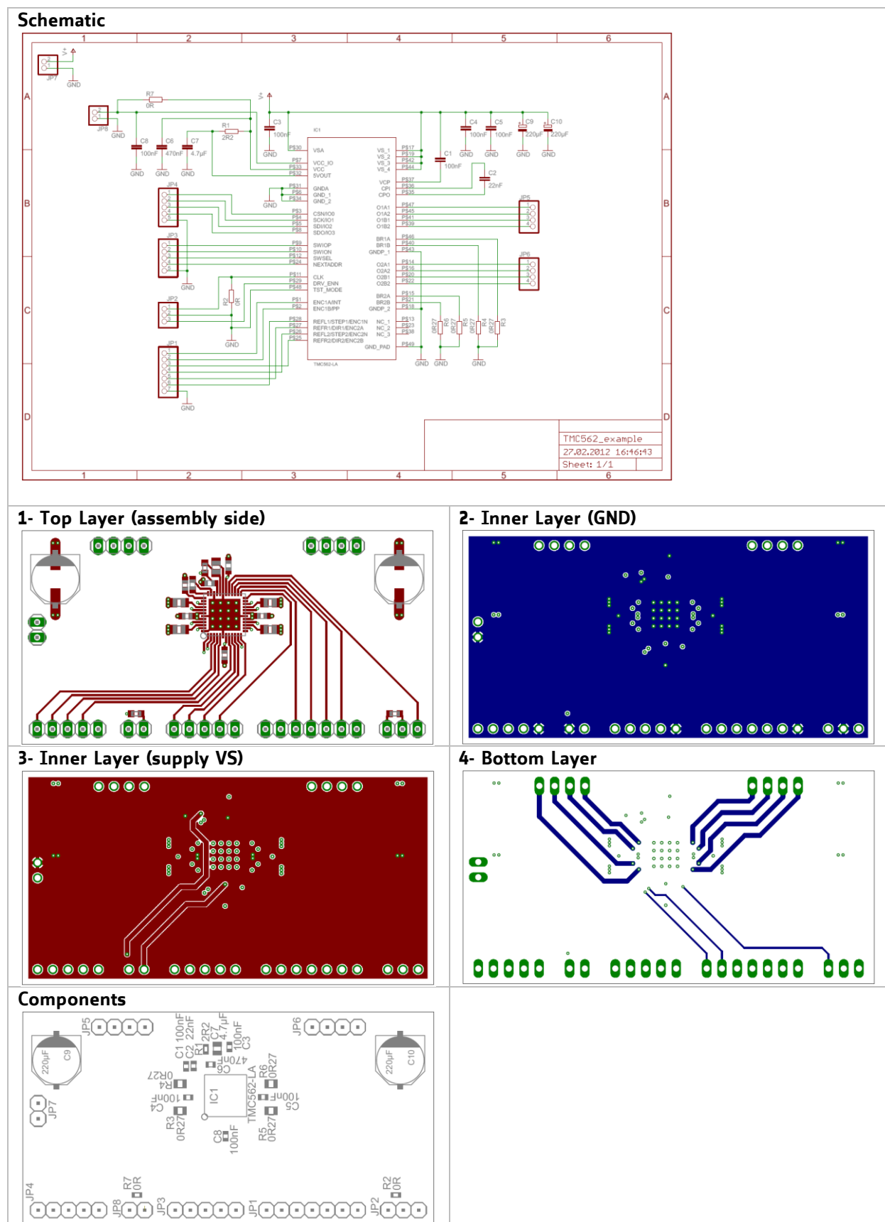
Figure 20.1 Layout example
