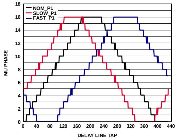
Figure 167. Mu Phase Characteristics of Three Devices from Different Process Lots at 1.2 GSPS
