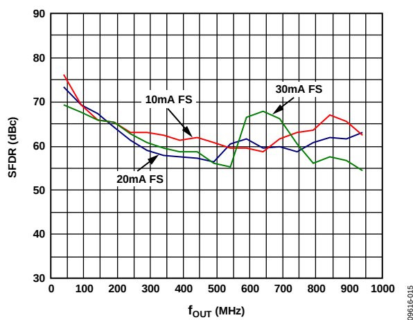
Figure 97. SFDR vs. f_{OUT} over DAC I_{OUTFS}
