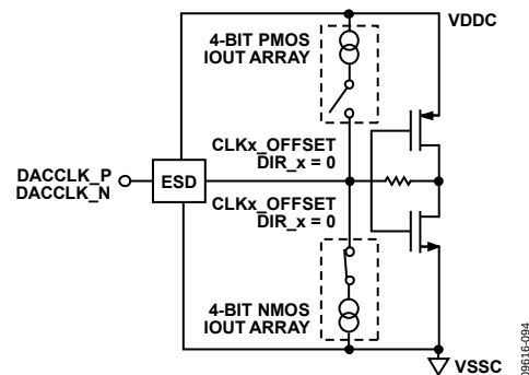
Figure 175. Clock Input and Common-Mode Control
