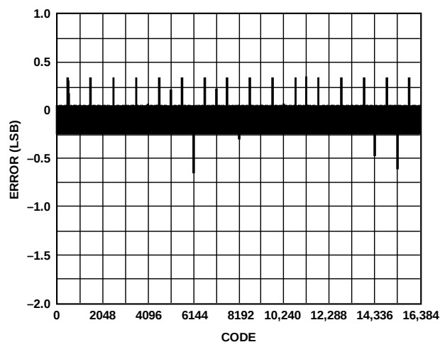
Figure 83. Typical DNL, 20 mA at 85°C
