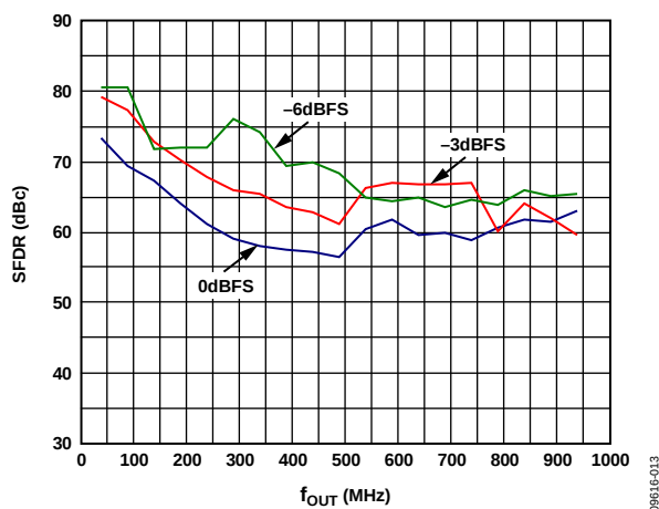
Figure 95. SFDR vs. f_{OUT} over Digital Full Scale
