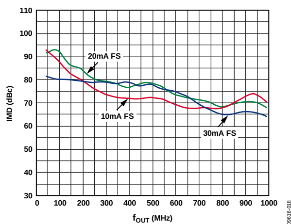
Figure 100. IMD vs. f_{OUT} over DAC I_{OUTFS}
