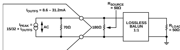
Figure 180. Equivalent Circuit for Determining Maximum Peak Power to a 50 \Omega Load
