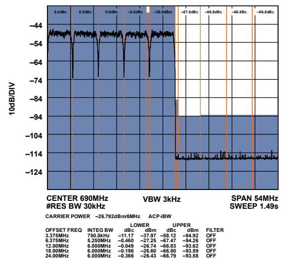
Figure 138. Mid Band Narrow-Band ACLR (Worse Side)
