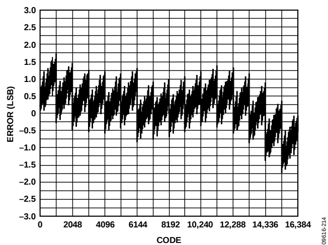
Figure 86. Typical INL, 30 mA at 25°C
