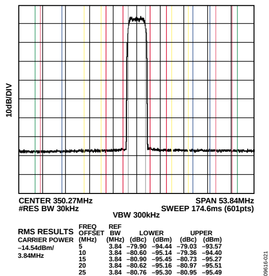
Figure 103. Single-Carrier WCDMA at 350 MHz, f_{DAC} = 2457.6 MSPS
