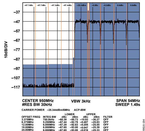
Figure 133. High Band Narrow-Band ACLR
