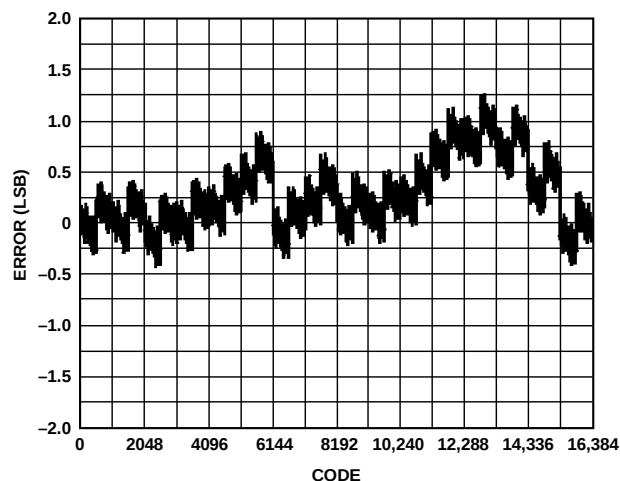
Figure 82. Typical INL, 20 mA at 85°C
