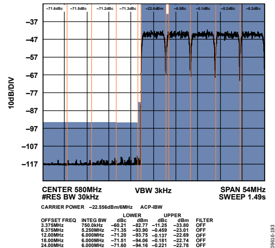
Figure 132. Mid Band Narrow-Band ACLR (Worse Side)
