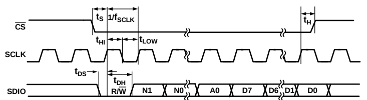
Figure 154. SPI Write Operation Timing
