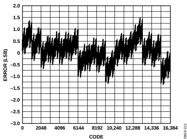
Figure 84. Typical INL, 10 mA at 25°C
