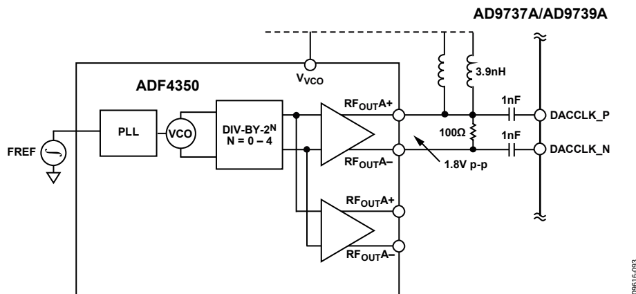
Figure 174. ADF4350 Interface to the AD9737A/AD9739A CLK Input
