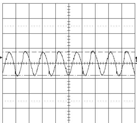
Output voltage ripple (50mV/div.) at T_{Pcb}=+25 °C, V_{in}=27 V, I_o=4.2 A resistive load with C=10 μF tantalum and 0.1 μF ceramic capacitors. Band width=20MHz. Time scale: 2 μs / div.
