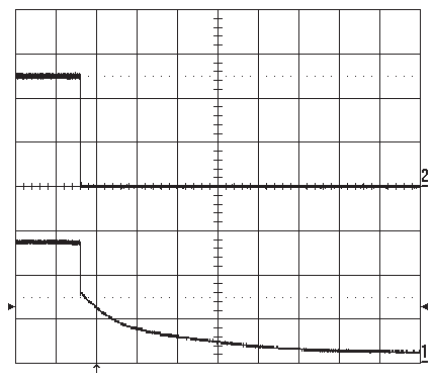
Turn-off at I_o=10A resistive load at T_{Pcb}=+25\text{ }^{\circ}C , V_{in}=27\text{ V} . Turn-off enabled by disconnecting V_{in} . Top trace: output voltage (10 V/div.). Bottom trace: input voltage (2 V/div.). Time scale: 10 ms/div.
