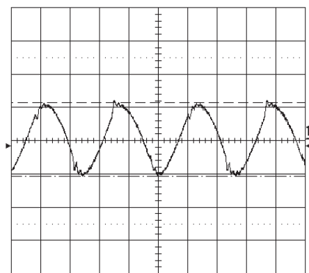
Output voltage ripple (50mV/div.) at T_{Pcb}=+25 °C, V_{in}=27 V, I_o=3.33 A resistive load with C=10 µF tantalum and 0.1 µF ceramic capacitors. Band width=20MHz. Time scale: 1 µs / div.
