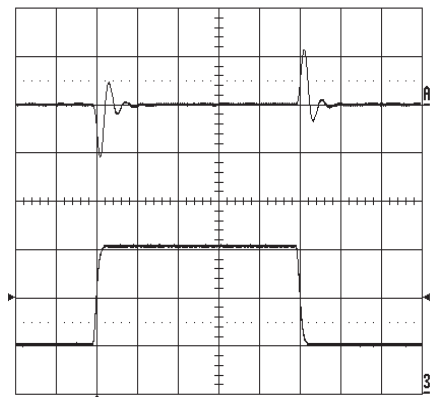
Output voltage response to load current step-change (2.5-7.5-2.5 A) at T_{Pcb}=+25\text{ }^{\circ}C , V_{in}=27\text{ V} . Top trace: output voltage (200mV/div.). Bottom trace: load current (2.5 A/div.) Time scale: 0.1 ms/div.
