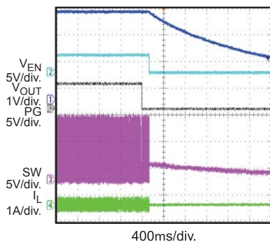
Shutdown through EN/SYNC I_{OUT}=0A
