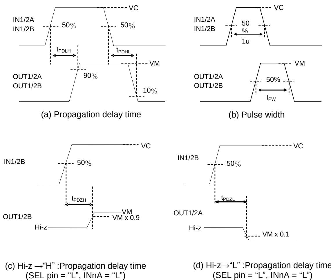
Figure 3. Time chart of propagation delay time and pulse width
