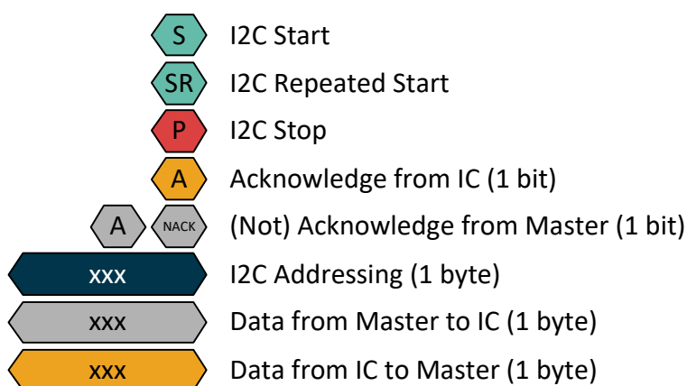
Figure 14: I 2 C Convention
