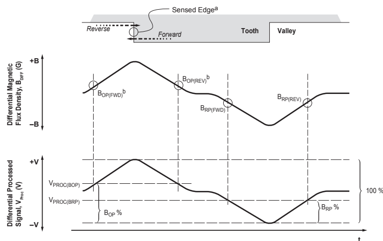
Figure 4: Definition of Terms for Switch Points
