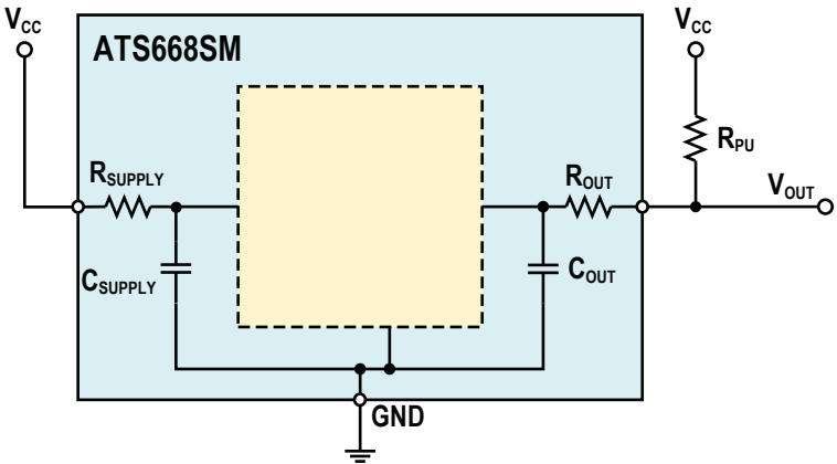
Figure 1: Typical Application
