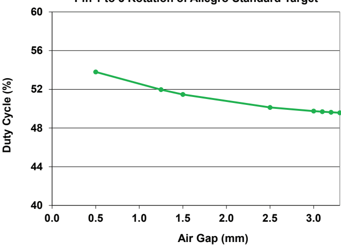
Average Duty Cycle versus Air Gap
